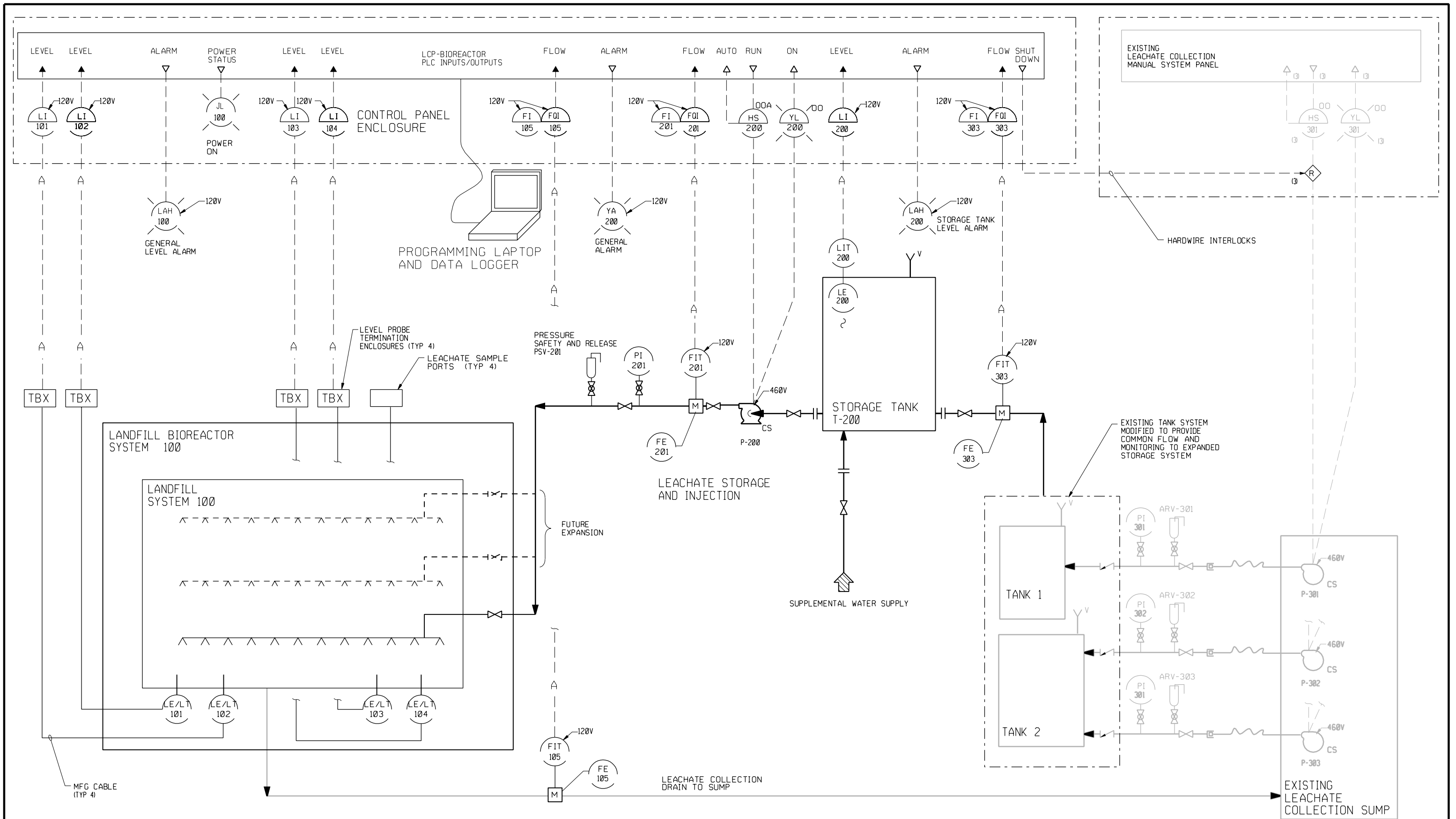
BIOREACTOR LANDFILL LEACHATE INJECTION AND REMOVAL SYSTEM
