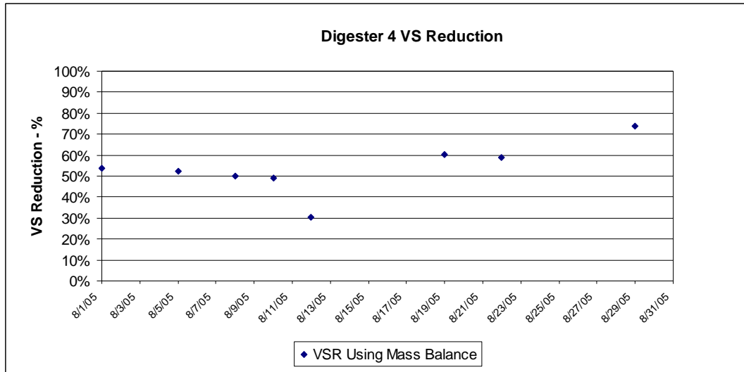
FIGURE 4-10 Digester 4 VS Reduction
