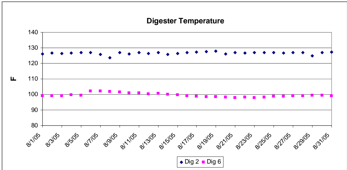
FIGURE 5-8 Digester Temperature
