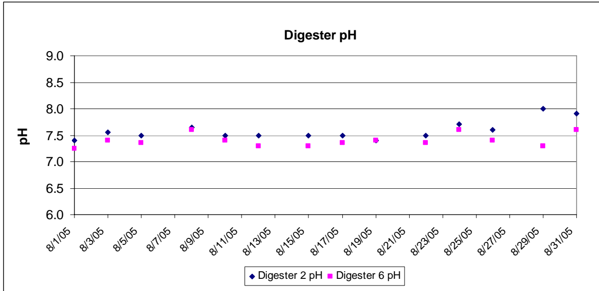
FIGURE 5-6 Digester pH
