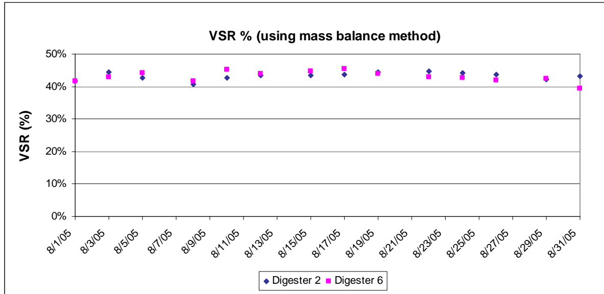
FIGURE 5-10 VS Reduction
