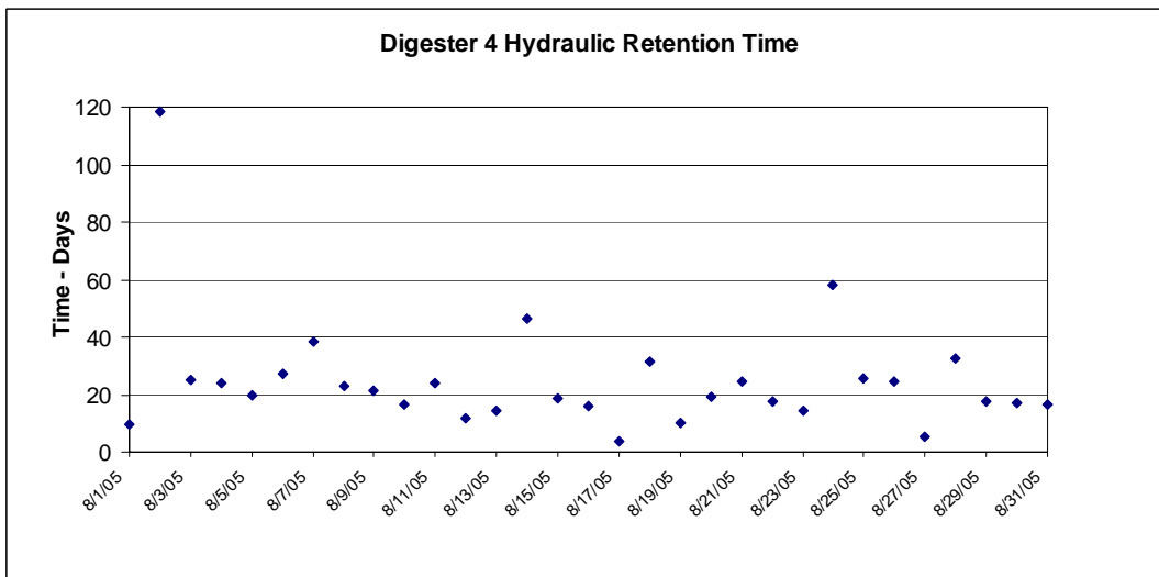
FIGURE 4-5 Digester 4 Hydraulic Retention Time
