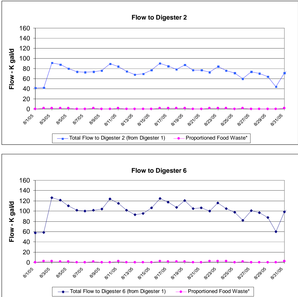
FIGURE 5-2 Biosolids and Food Waste Flow to Digesters 2 and 6
