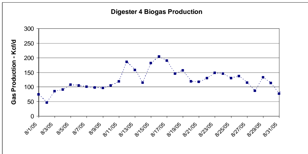
FIGURE 4-9 Digester 4 Gas Production
