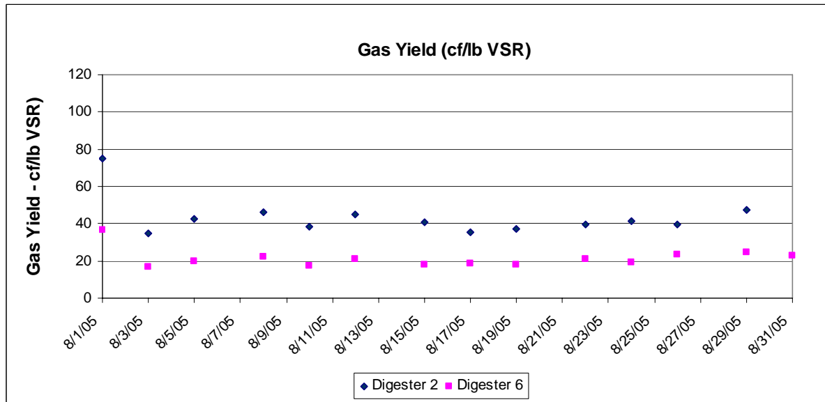
FIGURE 5-11 Biogas Yield
