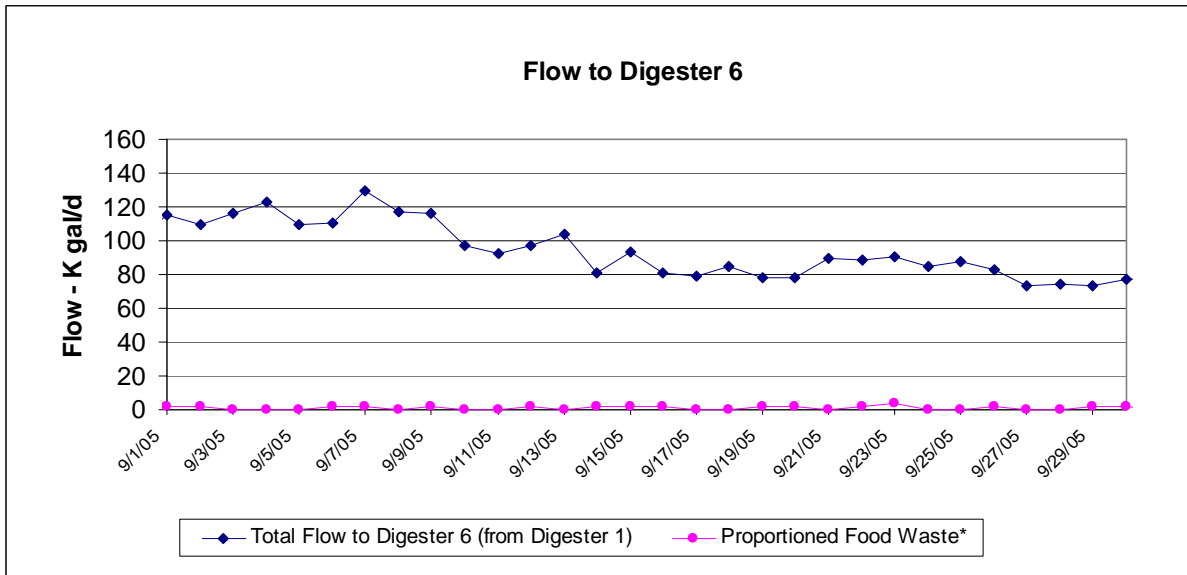
FIGURE 5-2 Biosolids and Food Waste Flow to Digesters 2 and 6
