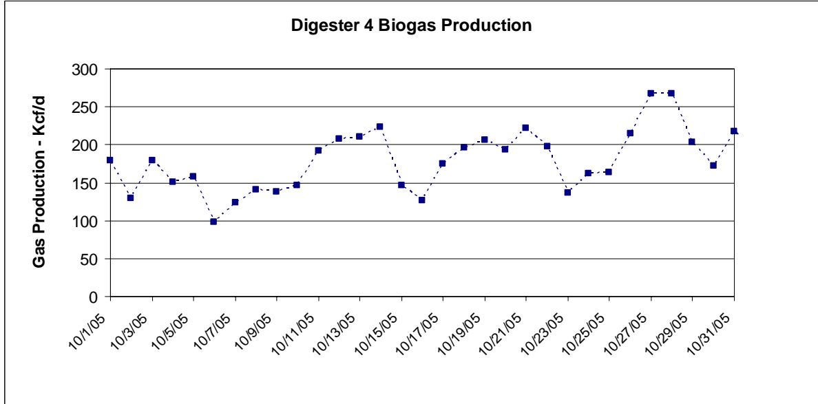
FIGURE 4-9 Digester 4 Gas Production
